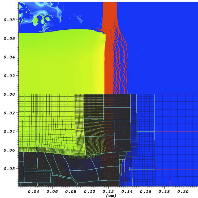
Figure 6: A typical current-day multiphysics simulation including vastly different physical regimes from hot vaporizing plasma to cold fragmented solid, all on a moving AMR mesh.
