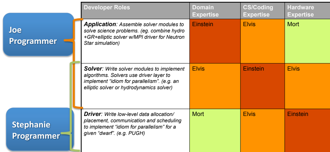
Figure 1: This diagram shows the stratification of developer roles and expertise on a complex code project. Domain experts were referred to as "Joe" programmers whereas the computer science experts were referred to as "Stephanie" programmers as shown on the left. The matrix on the right represents the expertise of these respective programmers in the areas of the science domain, numerical algorithms, and the low level details of computer architecture and tuning. A person is an "einstein" if they are an expert, an "elvis" who is conversant in the area, and an "mort" who is a non-expert. The programming environment offered to Joe may require a different set of criteria than the environment offered to Stephanie.
