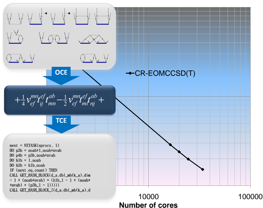
Figure 7: The Tensor Contraction Engine generates high-performance code from a high-level domain-specific language, thus reducing the coupling between application and architecture complexity into a relatively small translation layer. The resulting code has demonstrated excellent scaling to today’s largest machines.
