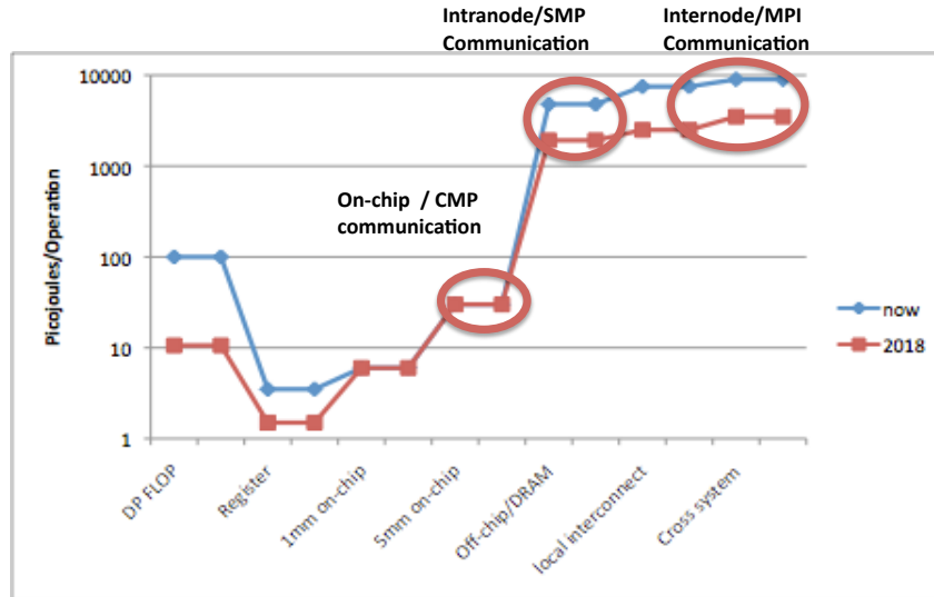
Figure 5: With new scaling rules and massive growth in parallelism, data locality is increasingly important. This diagram shows the cost of a double-precision multiply-add at different levels of the memory hierarchy (from the cost of performing the flop to the movement of data operands from registers, different distances on-chip, and distances off-chip.) The model of FPU and register access is based on the Tensilica LX2 core energy model, the energy consumed for cross-chip wires uses the Orion2 power model which is based on Balfour's model [6], memory access is based on the JEDEC DDRx memory roadmap, and cross-system is based on projections for VCSEL-based optical transceivers.
