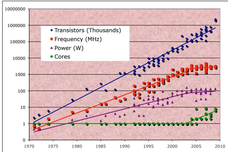
Figure 2: This graph shows that Moores law is alive and well, but the traditional sources of performance improvements (ILP and clock frequencies) have all been flattening. The performance of processors as measured by SpecINT has grown 52% per year with remarkable consistency, but improvements tapered off around 2003 due to the end of Dennard scaling rules. ( This figure is based on original data from Kunle Olukotun and Herb Sutter, but updated with more recent data. )
