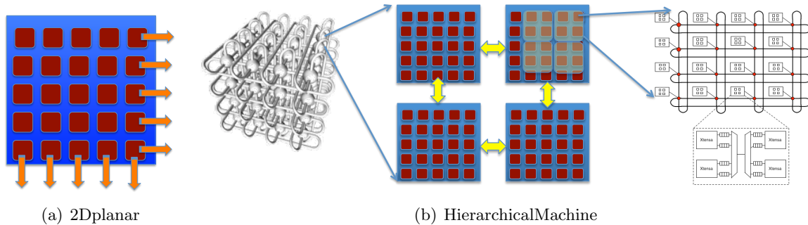
Figure 4: As the number of computational elements per chip scale to hundreds of endpoints, Networks-on-chip are expected to adopt constrained topologies (meshes or torus) as they scale out a 2D planar geometry with hundreds of processing elements [54, 61]. The abstract machine model may need to include notions of hierarchy or even topology for effective management of horizontal data locality.
