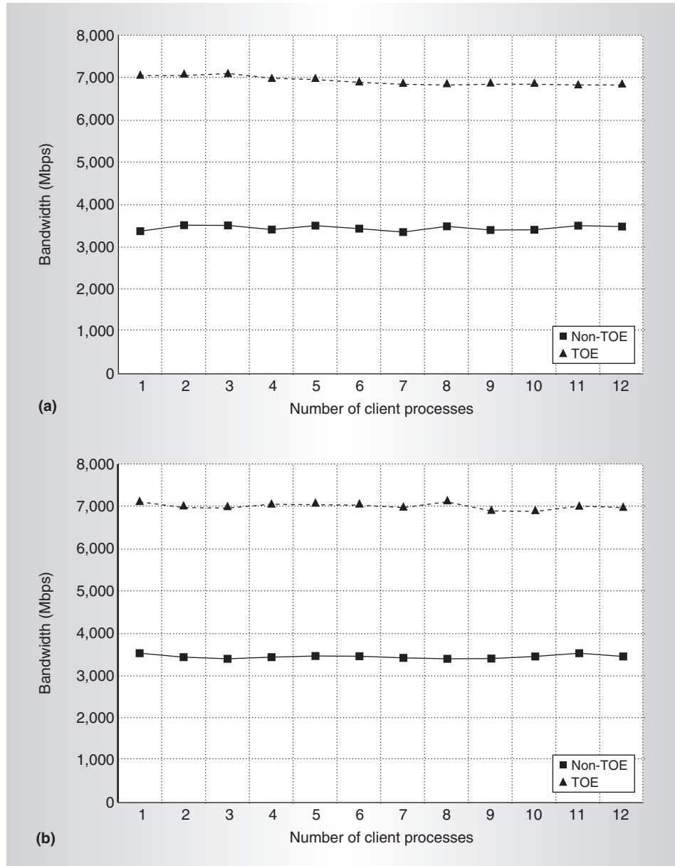
Figure 6. Fan-out (a) and fan-in (b) bandwidth tests.
