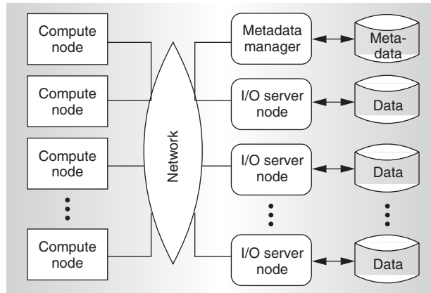
Figure 10. Typical PVFS environment.
