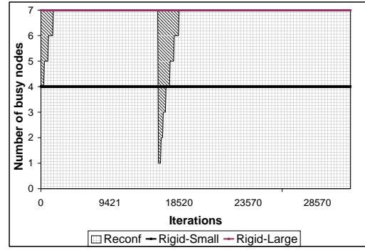
Figure 7. Node Utilization for Reconf (a) Burst Length = 1K and (b) Burst Length = 16K
