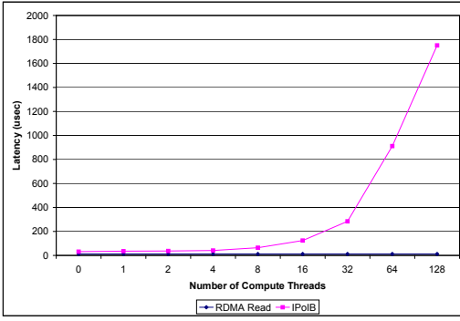
Figure 5. Performance of iPoIB and RDMA Read with background load: (a) Latency, (b) Bandwidth
