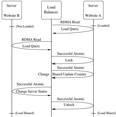
Figure 1. RDMA based Protocol for Dynamic Reconfigurability
