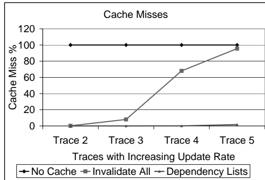
Figure 9. Cache Misses With Increasing Update Rate
